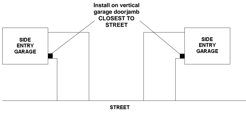
FIGURE 3 - SIDE ENTRY garage mounting location.
